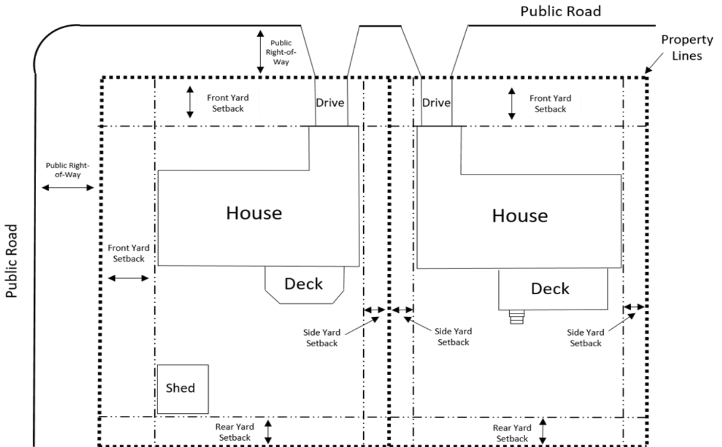
Setback Diagram
